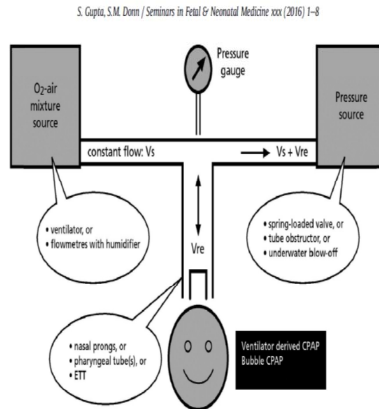
Fig. 3. Continuous-flow positive airway pressure (CPAP) system. ETT, endotracheal tube.
